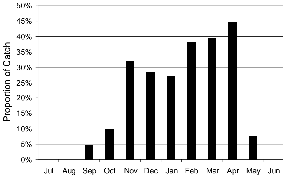
Fig. 9. Seasonal variation (Jan. 2003 – Dec. 2006) in proportion of catch for razorback sucker with physical wounds suggesting avian predation. No surveys occur during summer months. Data show a general increase in such wounds during winter-spring months when over-wintering migratory avian piscivores are abundant in the lower Colorado River, AZ-CA.
